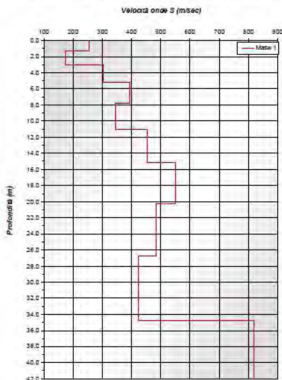
Shear-Wave Velocity Profile from Surface waves inversion
