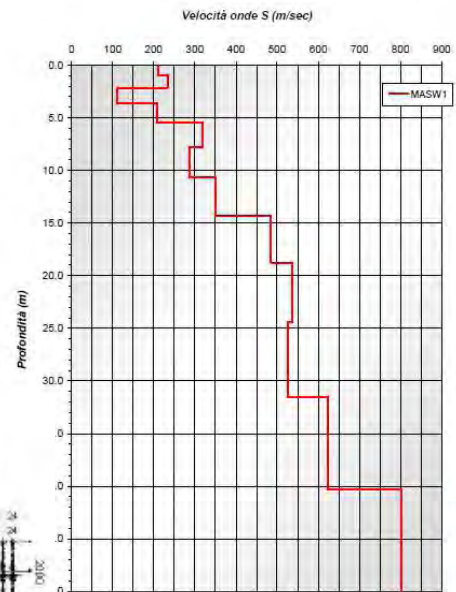
Shear-Wave Velocity Profile from Surface waves inversion
